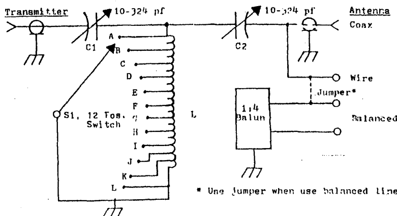
MFJ-901B Circuit Diagram
